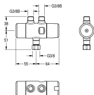
THERMOSTATIC MIXING VALVE
